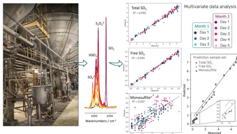
Figure 1: Raman spectra were collected along the chemical recovery chain (cascade of Venturi scrubbers). Different components in the scrubber media are identified via their distinct spectral fingerprint. Multivariate data analysis allows determination of several target variables (total SO 2 , free SO 2 , monosulfite) from a single Raman spectrum. Cross-validation and prediction results of the multivariate model based on at-line measurements yield a reliable model performance .
